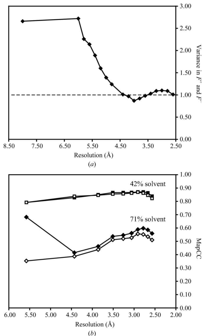
Figure 3 Analysis of the anomalous signal and determination of the hand of the \text{Ta}_6\text{Br}_{12}^{2+} -substructure enantiomorph. (a) Plot of variance in F^+ and F^- versus resolution. The \text{Ta}_6\text{Br}_{12}^{2+} anomalous signal obtained from the Derivative-1 data set decreased rapidly beyond 5.5 Å resolution. The dashed line represents random variance in F^+ and F^- . (b) SHELXE map correlation coefficient (MapCC) versus resolution. Final MapCCs after 100 cycles of density modification are given for the original enantiomorph and 71% solvent content (filled diamonds), the inverted enantiomorph and 71% solvent content (open diamonds), the original enantiomorph and 42% solvent content (filled squares) and the inverted enantiomorph and 42% solvent content (open squares).
