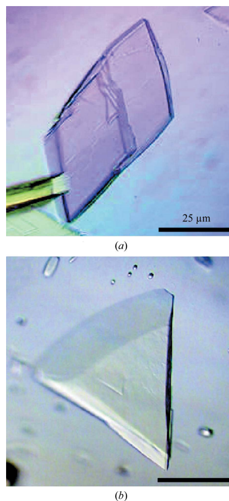
Figure 1 Images of representative crystals of the C2 (a) and C22 21 (b) crystal forms of LdcI. Scale bars correspond to 25 μm.
